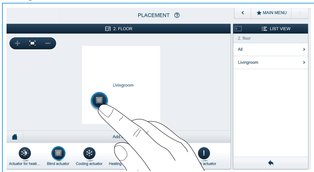
Fig. 7: Adding device
