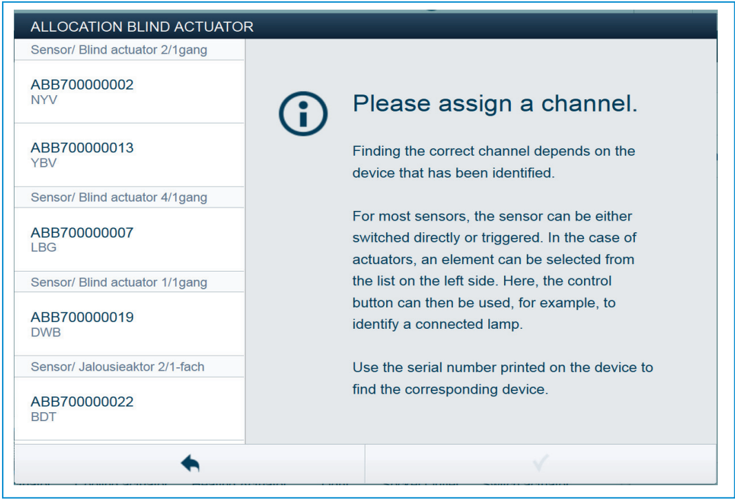
Fig. 8: Allocation
