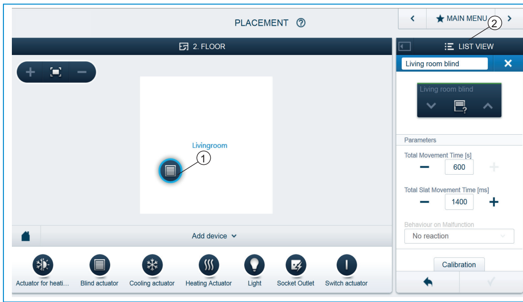
Fig. 12: Device selection
